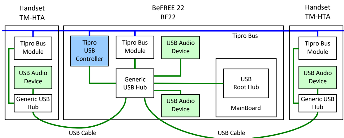
Figure 11 - Example BeFREE 22 Configuration – Schematic Representation
